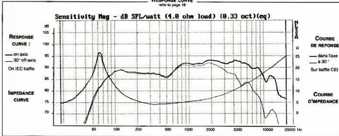
RESPONSE CURVE refer to page 18
